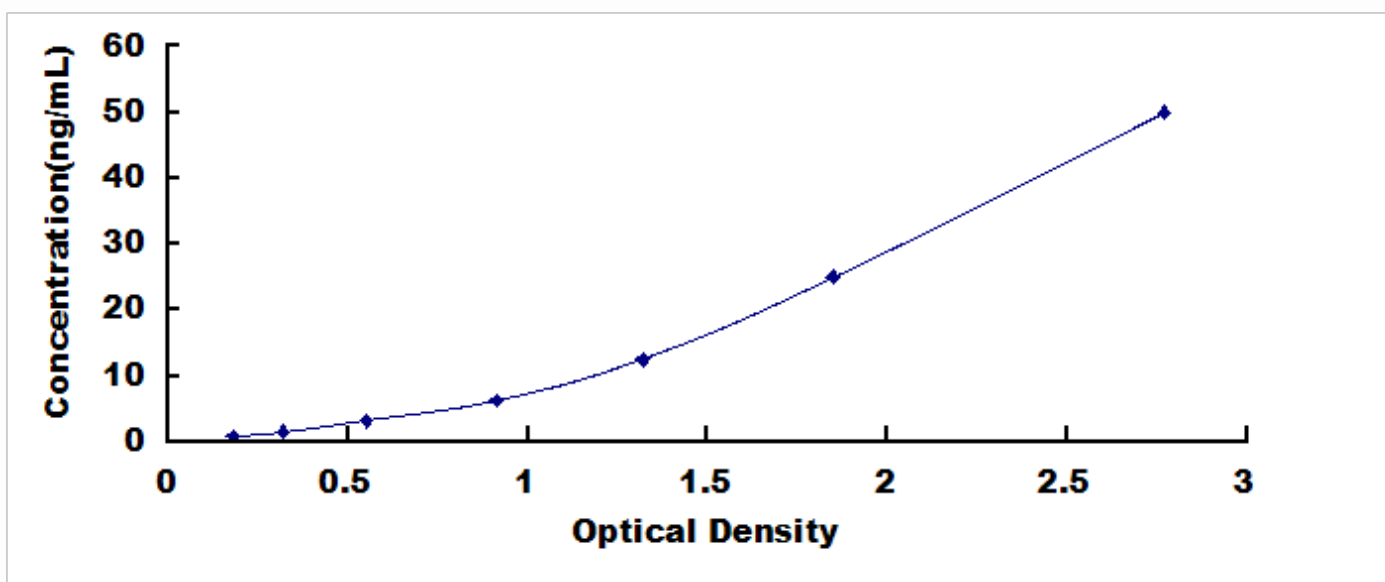
Typical Standard Curve for Dermcidin, Human ELISA.
