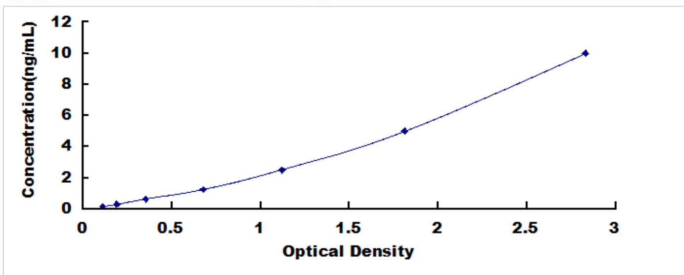
Typical Standard Curve for ENA78, Human ELISA.
