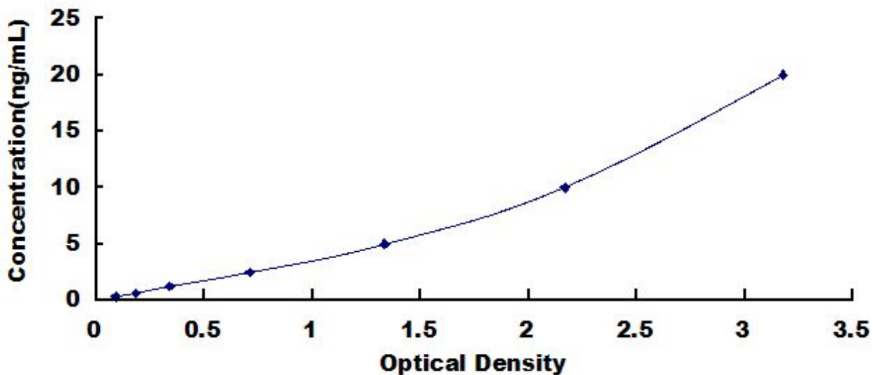
Typical Standard Curve for Fascin, Human ELISA.
