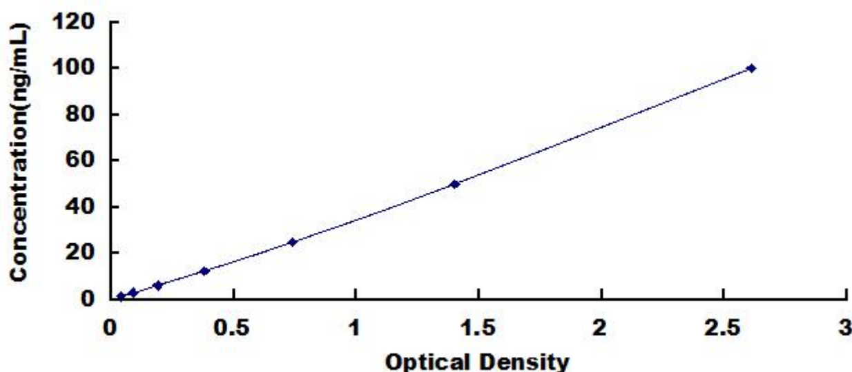
Typical Standard Curve for GAL2, Human ELISA.
