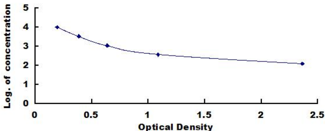
Typical Standard Curve for Ghrelin, Mouse ELISA.
