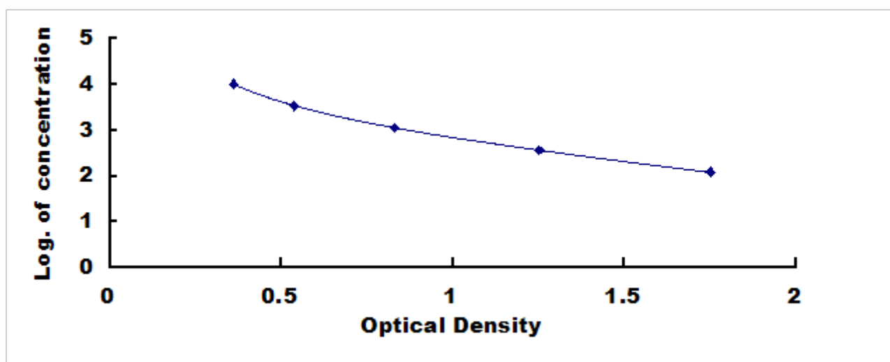
Typical Standard Curve for GA ELISA.
