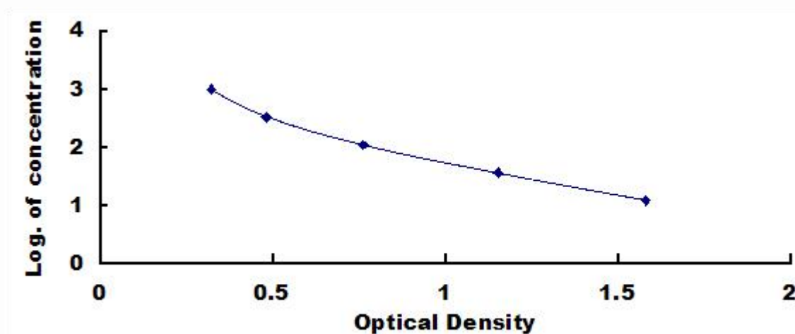
Typical Standard Curve for GLP1, Mouse ELISA.
