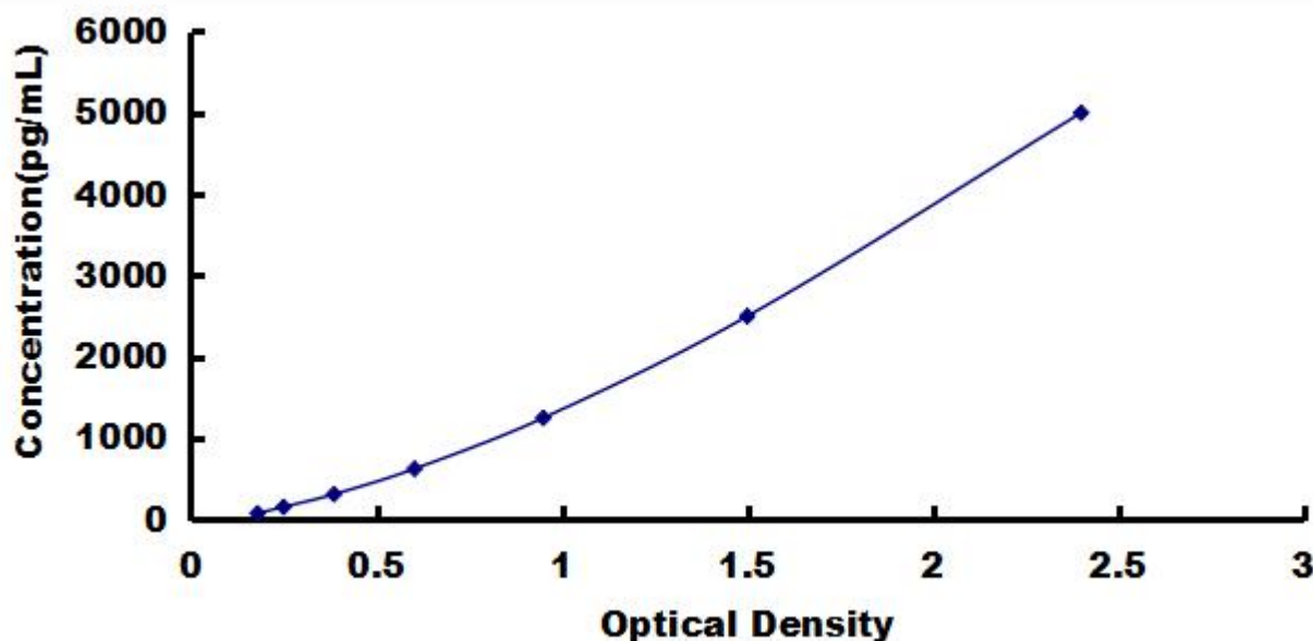
Typical Standard Curve for GLO1, Mouse ELISA.
