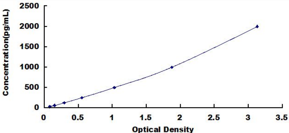
Typical Standard Curve for Granulin, Mouse ELISA.
