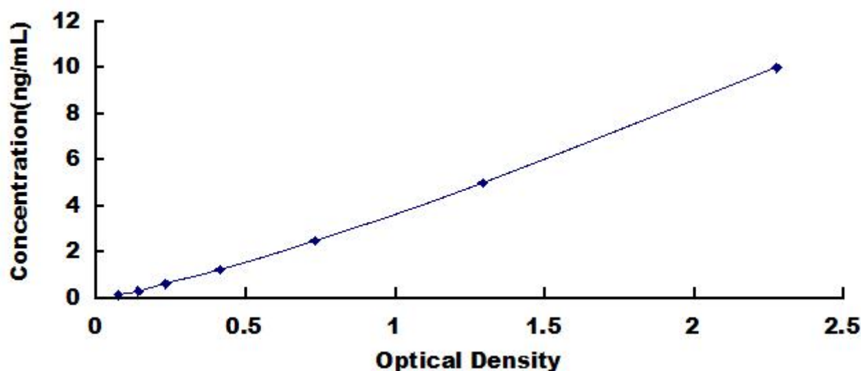
Typical Standard Curve for HIF1a, Human ELISA.
