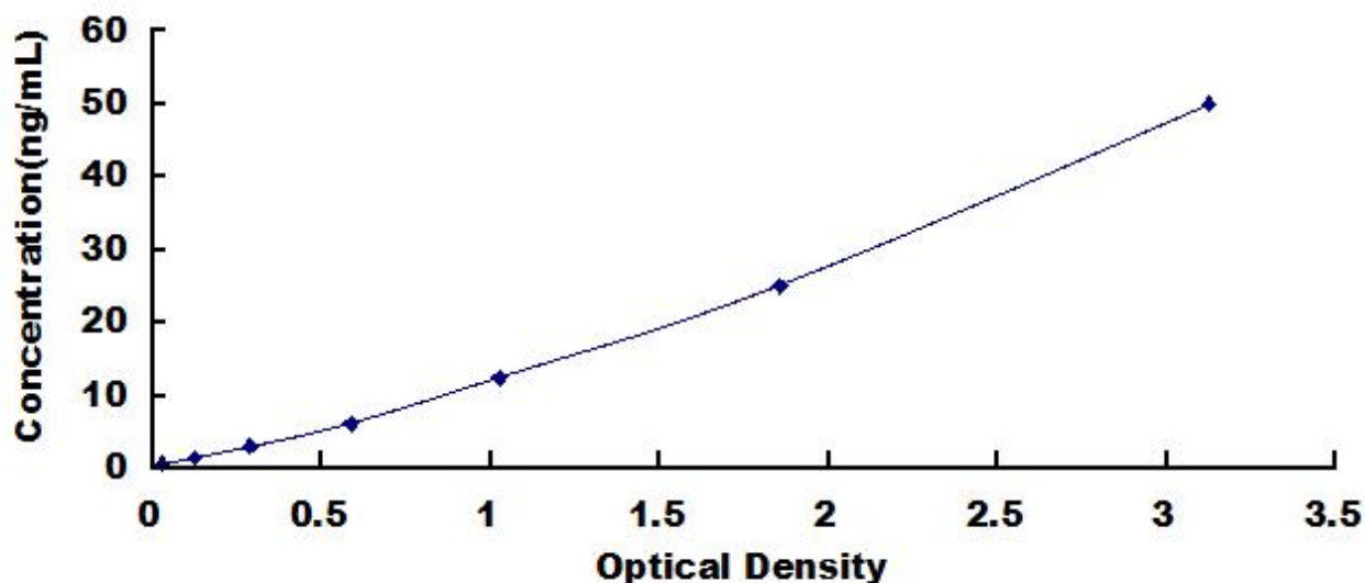
Typical Standard Curve for IGF1, Bovine ELISA.
