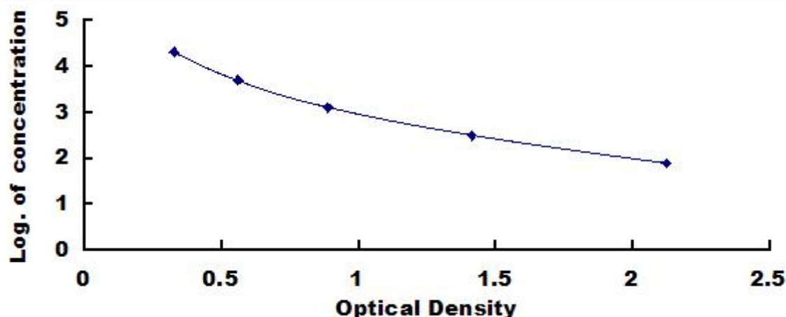
Typical Standard Curve for Lysophosphatidylcholine ELISA.
