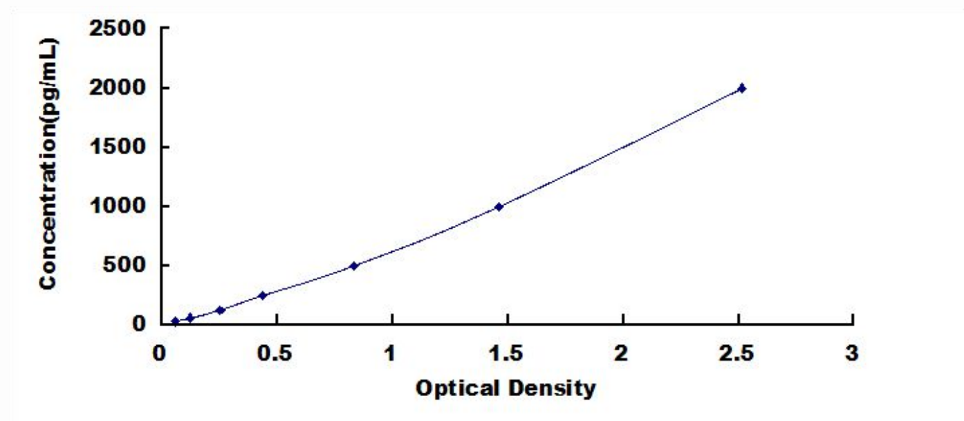
Typical Standard Curve for MIF, Rat ELISA.
