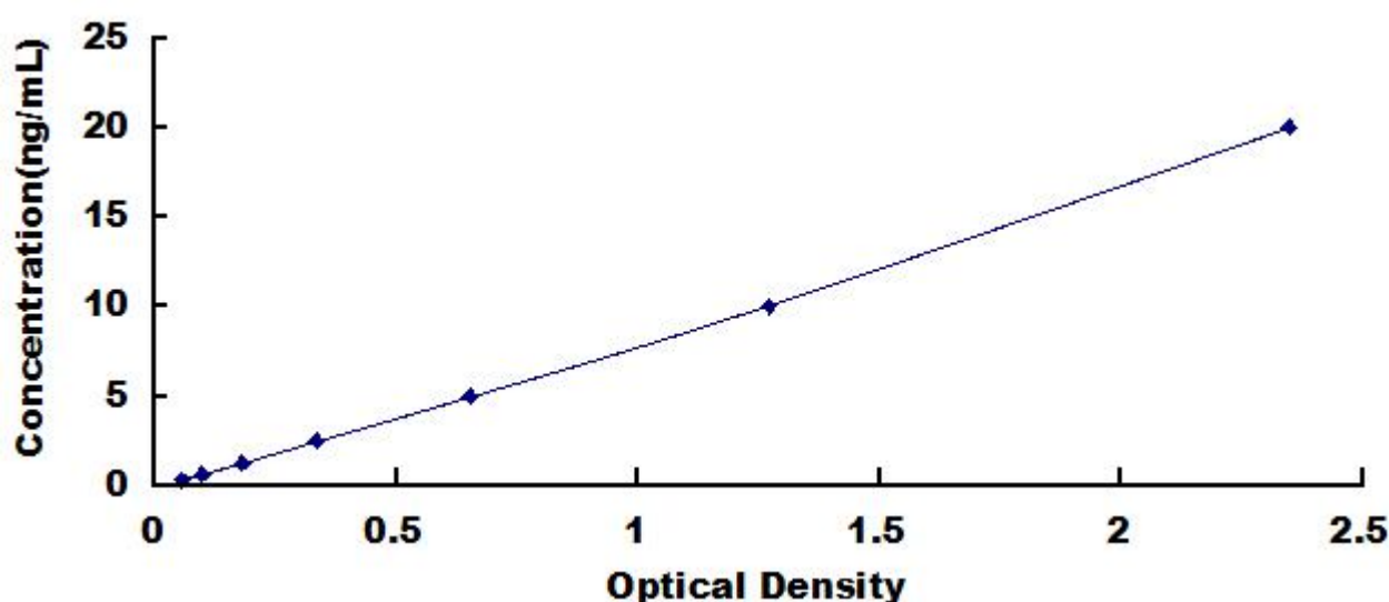
Typical Standard Curve for MMP2, Human ELISA.
