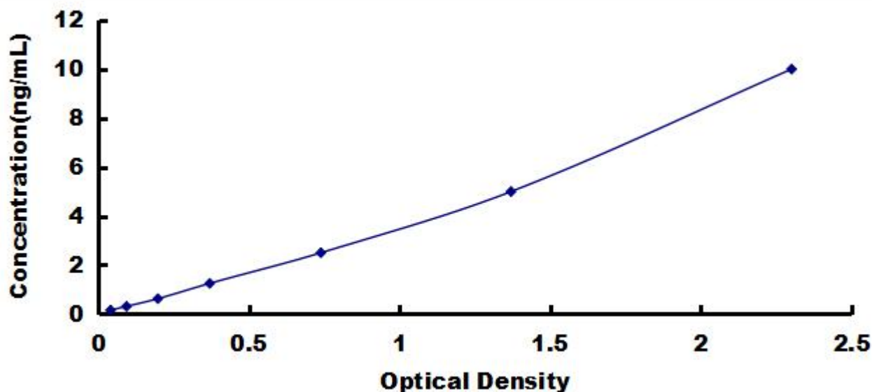
Typical Standard Curve for METRN, Human ELISA.
