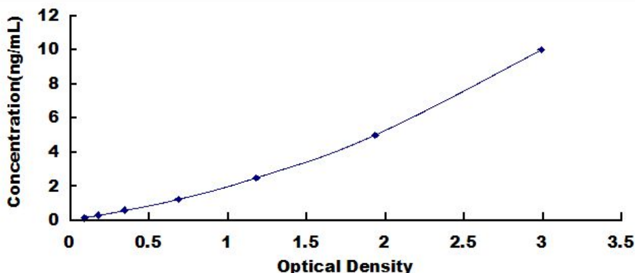
Typical Standard Curve for MFN2, Human ELISA.
