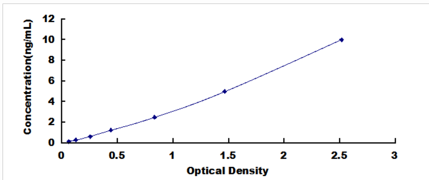
Typical Standard Curve for Smad2 ELISA.
