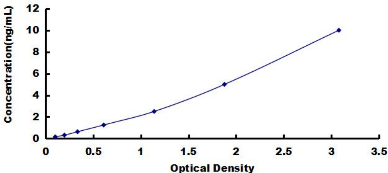
Typical Standard Curve for MYBPC3, Human ELISA.
