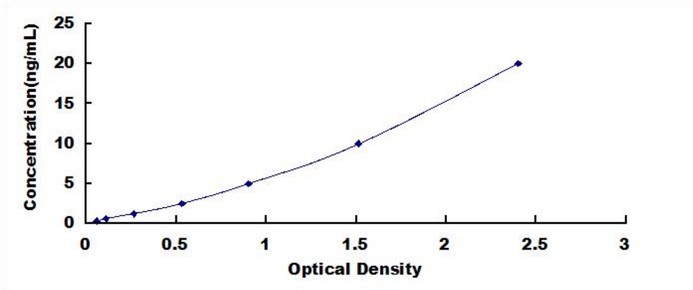
Typical Standard Curve for NRG4, Mouse ELISA.
