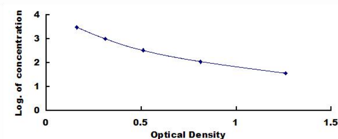
Typical Standard Curve for Neurotensin, Rat ELISA.
