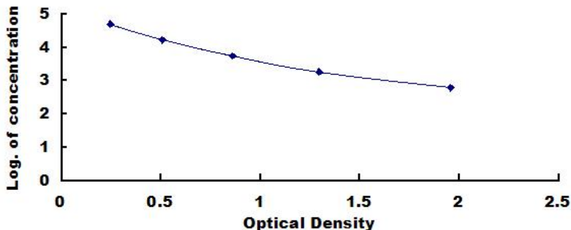
Typical Standard Curve for Ouabain ELISA.
