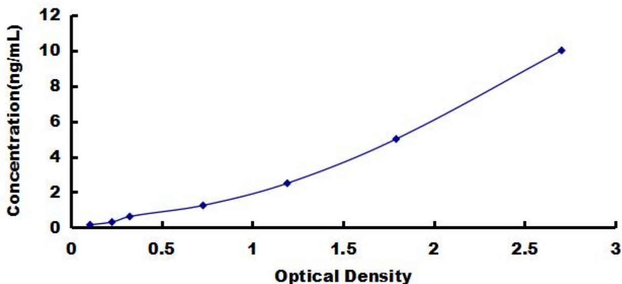
Typical Standard Curve for PPARgC1a, Mouse ELISA.
