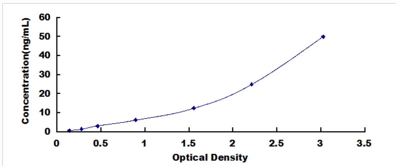
Typical Standard Curve for Podocin, Human ELISA.
