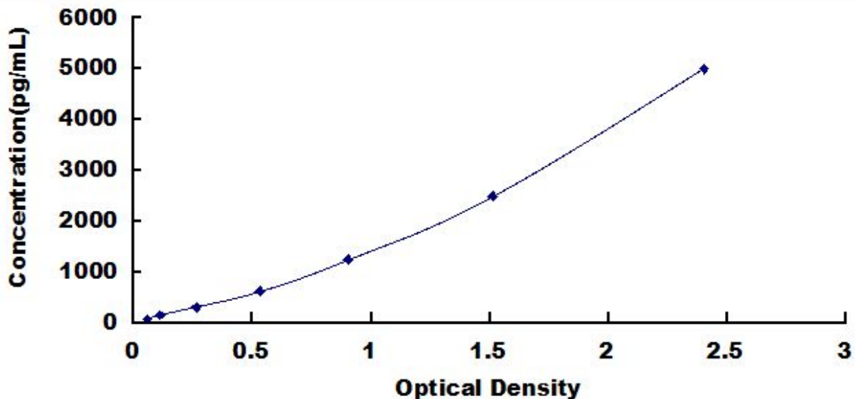
Typical Standard Curve for Prestin, Mouse ELISA.
