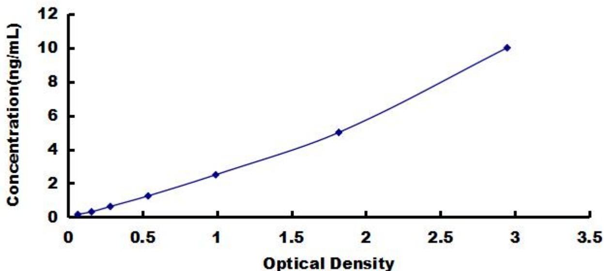
Typical Standard Curve for PRNP, Bovine ELISA.
