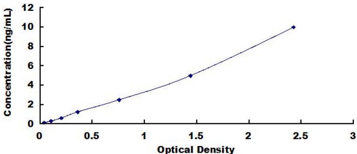
Typical Standard Curve for PLOD2, Human ELISA.
