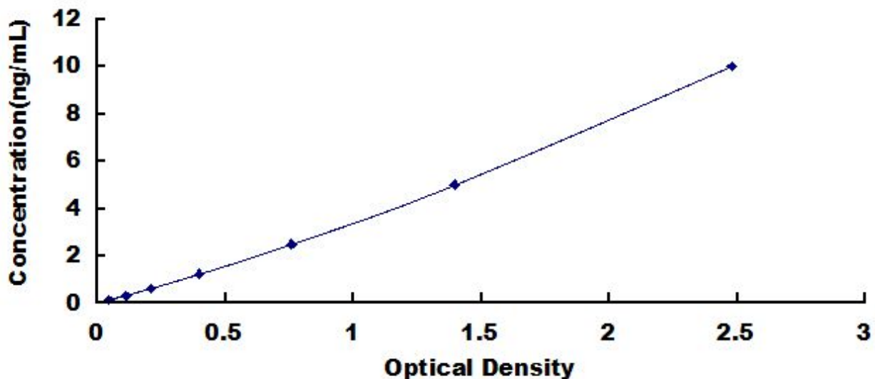
Typical Standard Curve for SERT, Human ELISA.
