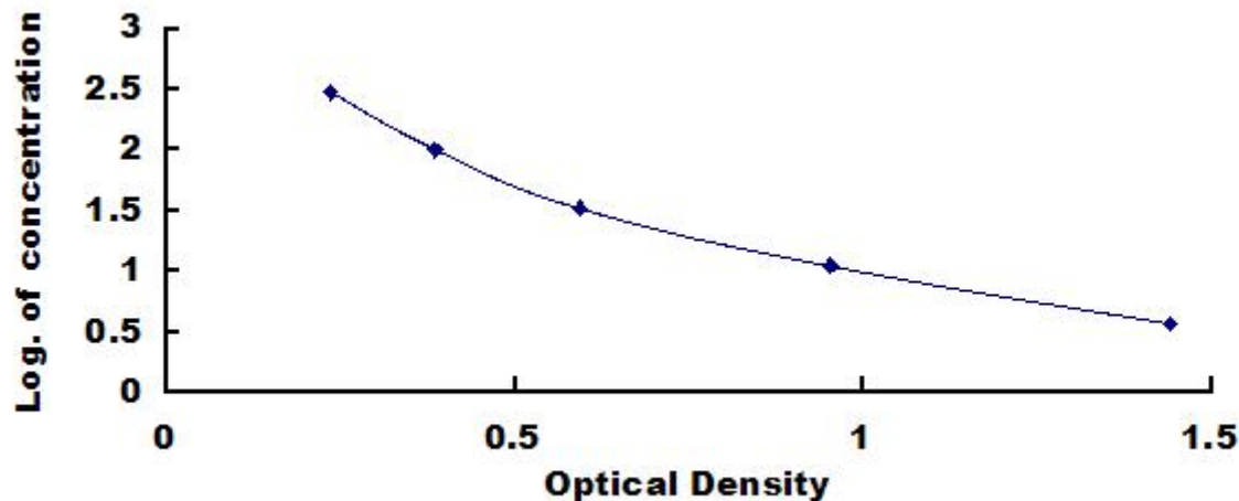
Typical Standard Curve for T4 ELISA.
