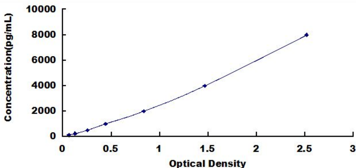
Typical Standard Curve for TFR, Human ELISA.
