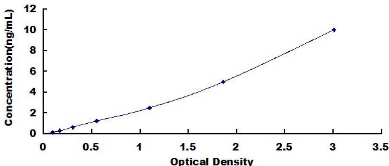
Typical Standard Curve for TRA2b, Human ELISA.
