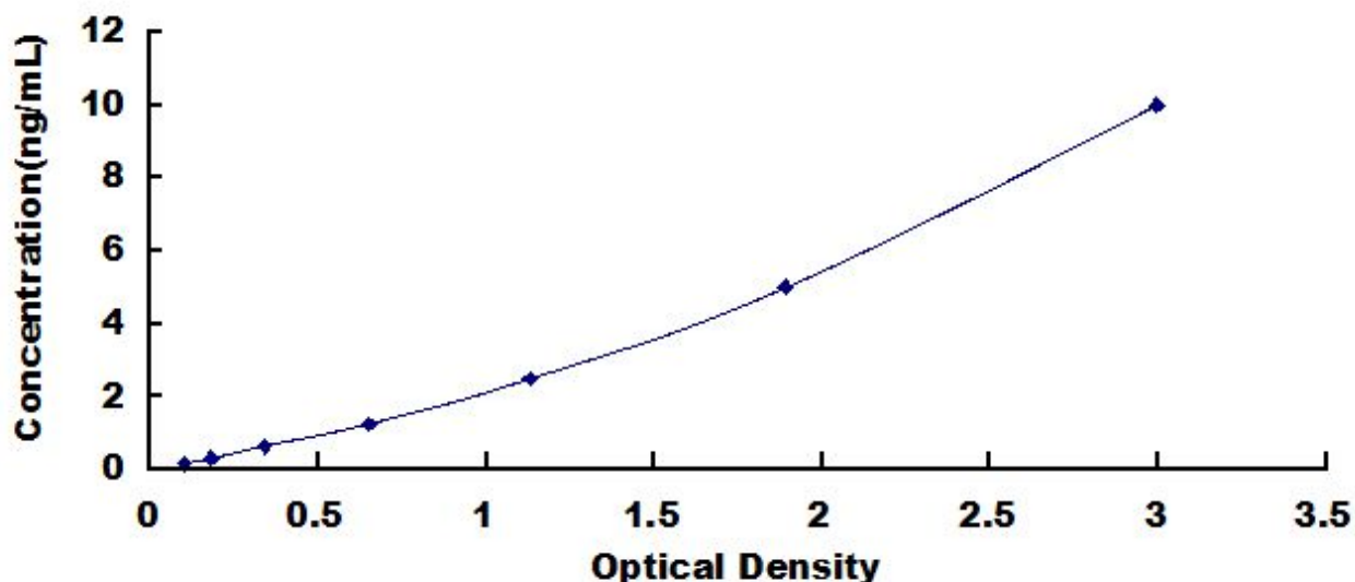
Typical Standard Curve for Uromodulin, Mouse ELISA.
