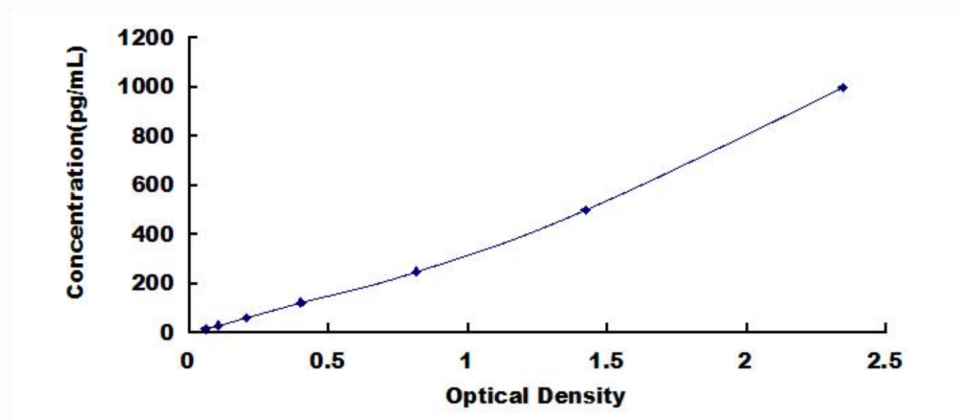
Typical Standard Curve for VEGF165, Human ELISA.
