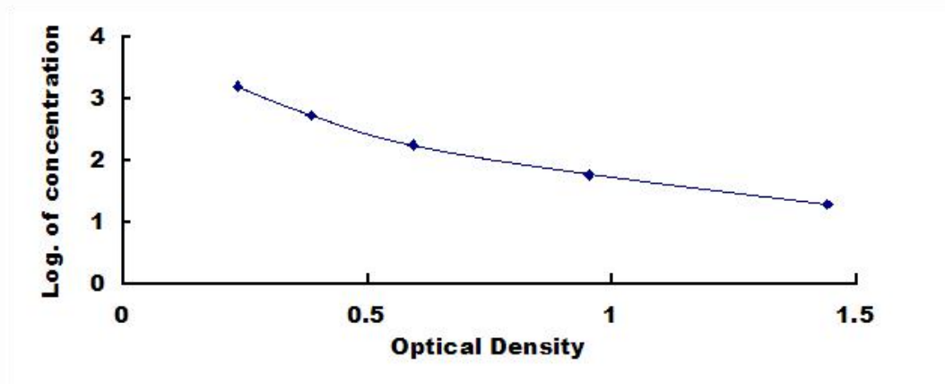
Typical Standard Curve for AGE ELISA.
