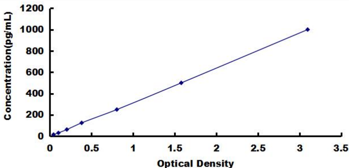
Typical Standard Curve for IL1a, Mouse ELISA.
