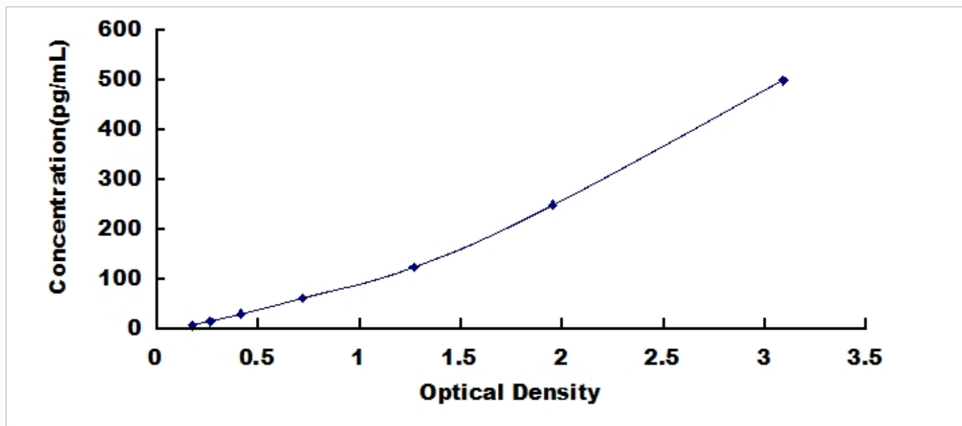
Typical Standard Curve for IL27, Mouse ELISA.
