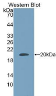
Figure. Western Blot; Sample: Recombinant ADM, Human.
