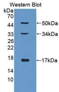
Figure. Western Blot; Sample: Recombinant COL10, Human.
