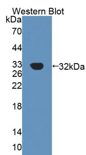
Figure. Western Blot; Sample: Recombinant CAR, Mouse.
