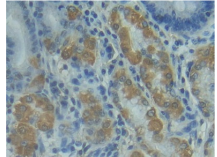
DAB staining on IHC-P; Samples: Human Stomach Tissue; Primary Ab: 20µg/ml Rabbit Anti-Human FASL Antibody Second Ab: 2µg/mL HRP-Linked Caprine Anti-Rabbit IgG Polyclonal Antibody (Catalog: SAA544Rb19)
