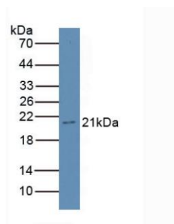
Figure. Western Blot; Sample: Rat Stomach Tissue.
