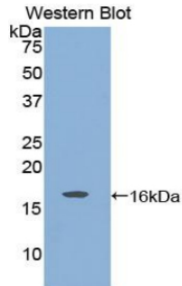
Figure. Western Blot; Sample: Recombinant GDNF, Rat.
