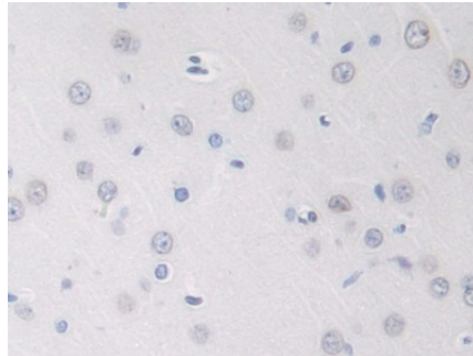
DAB staining on IHC-P; Samples: Rat Cerebrum Tissue; Primary Ab: 10µg/ml Rabbit Anti-Rat GDNF Antibody Second Ab: 2µg/mL HRP-Linked Caprine Anti-Rabbit IgG Polyclonal Antibody (Catalog: SAA544Rb19)
