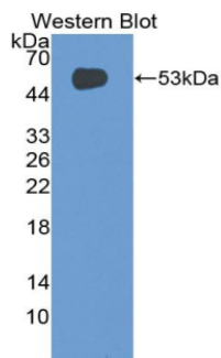
Figure. Western Blot; Sample: Recombinant GP9, Rat.
