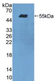
Figure. Western Blot; Sample: Recombinant ITGa9, Human.
