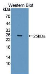
Figure. Western Blot; Sample: Recombinant ITIH5, Mouse.
