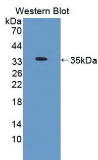
Figure. Western Blot; Sample: Recombinant IL1b, Bovine.
