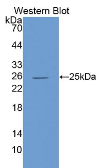
Figure. Western Blot; Sample: Recombinant IL6, Simian.
