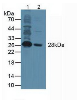
Figure. Western Blot; Lane1: Human Umbilical Cord Tissue; Lane2: Human Placenta Tissue.
