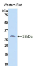
Figure. Western Blot; Sample: Recombinant Smad3, Mouse.
