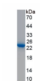
Figure. SDS-PAGE
