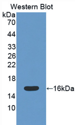
Used in Western Blot, Sample: Recombinant CAT, Mouse
